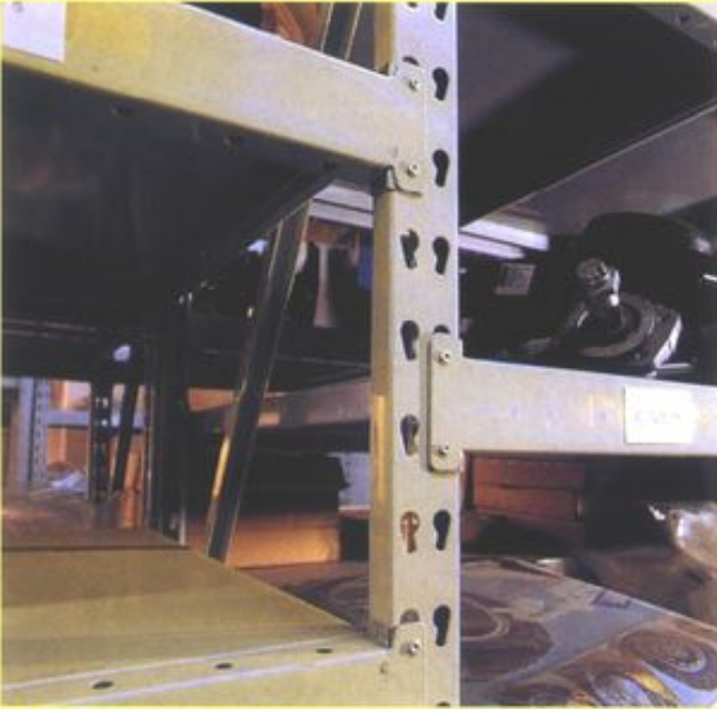
DETALLE ENGANCHE E-40 DETAIL CONECTION E-40
