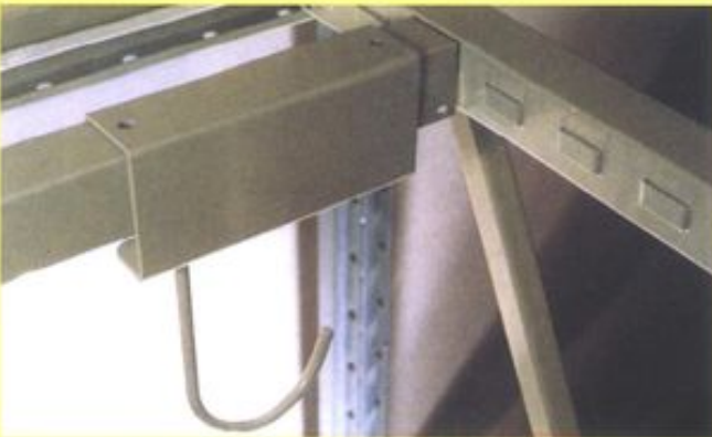
DETALLE GANCHO CHAPA DETAIL CAR BODY PARTS HOOK
