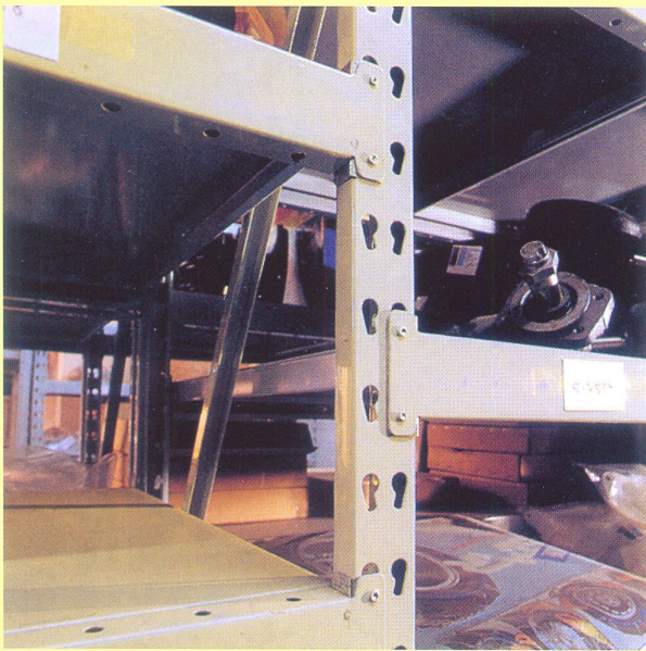
DETALLE ENGANCHE E-40 DETAIL CONECTION E-40
