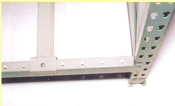
DETALLE FIJACION AL-40 DETAIL FASTENING LONGITUDINAL SUPPORT
